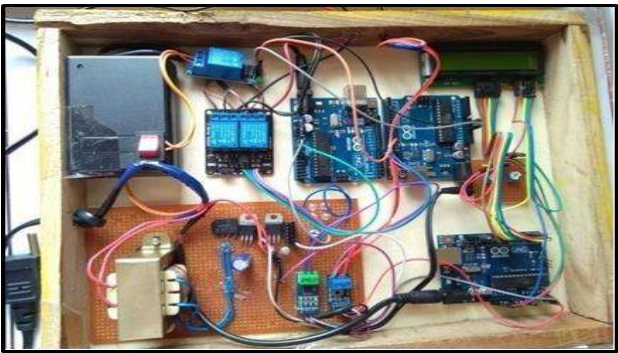
Fig. 4.2 Circuit Module of Proposed System
