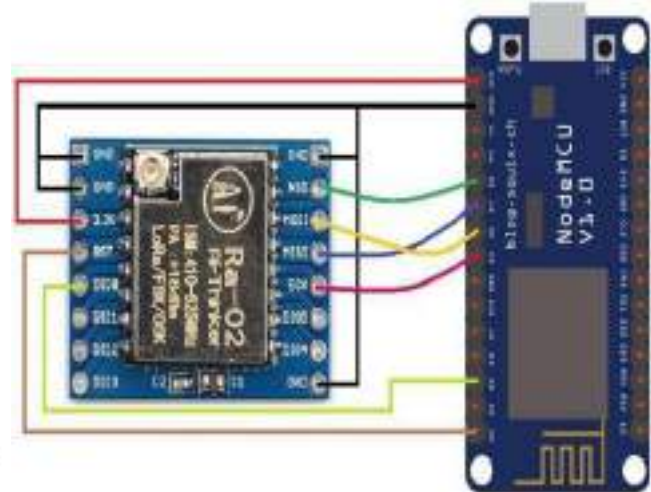
Figure3: Receiver Side
