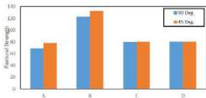
Fig.10: Flexural Strength
