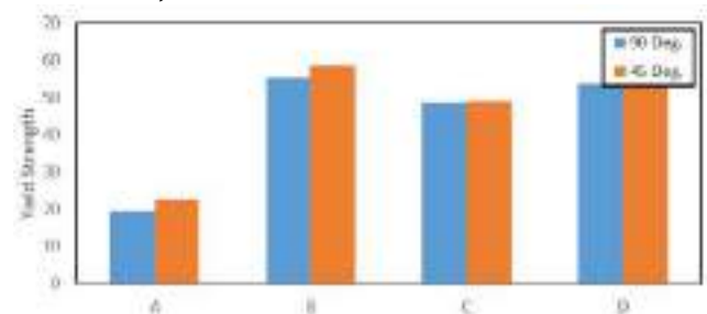
Fig.5: Yield Strength
