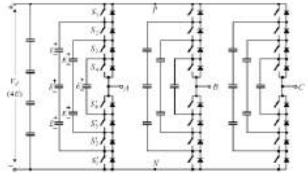
Fig 4.1 Five-level flying-capacitor inverter
