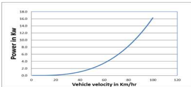
Figure 2. Velocity of a vehicle vs P_{ad}
