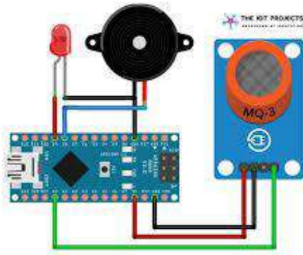
Fig 2. Circuit Diagram
