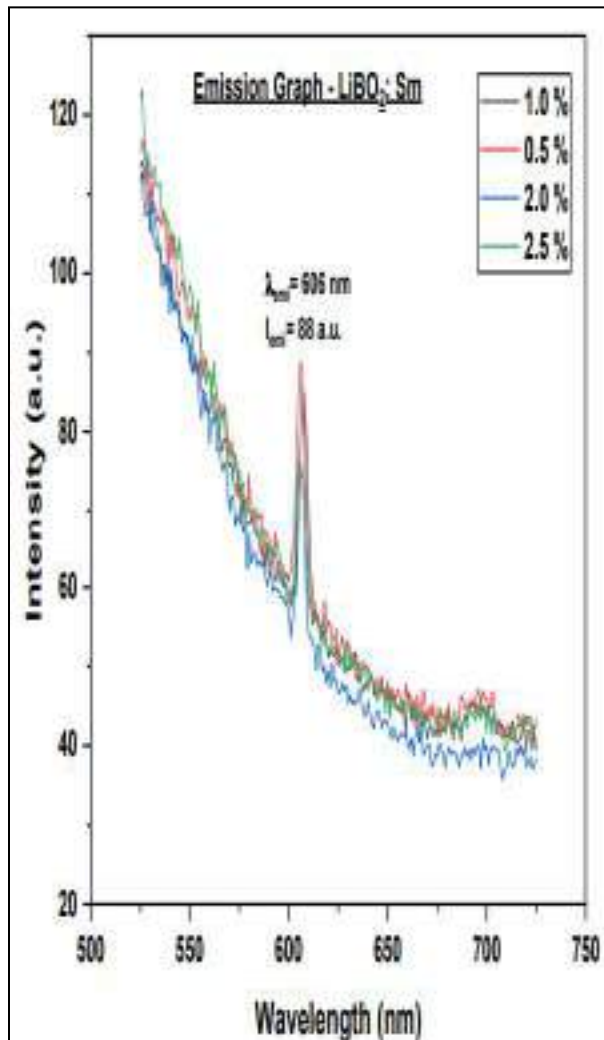
Figure 1(B): Emission graph – \text{LiBO}_2:\text{Sm}^{3+}
