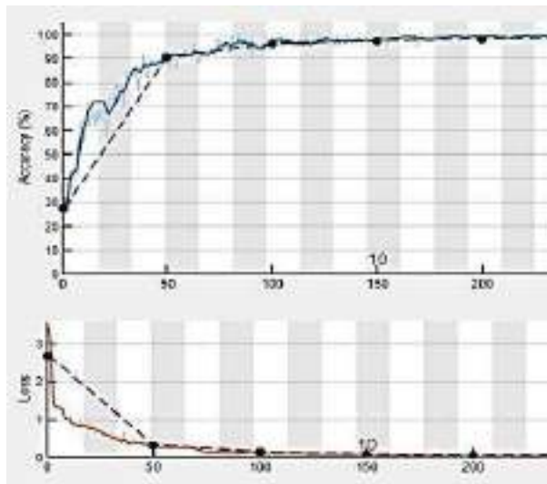
Figure 2. Training accuracy & Loss in SqueezeNet
