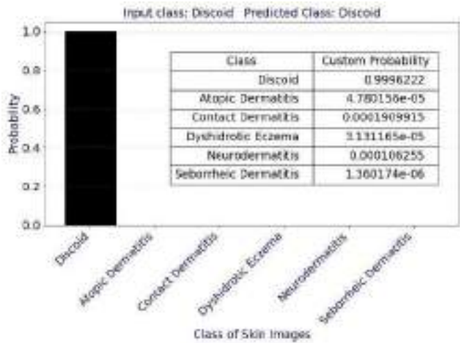
Fig.8(c)ProbabilitiesofClasses
