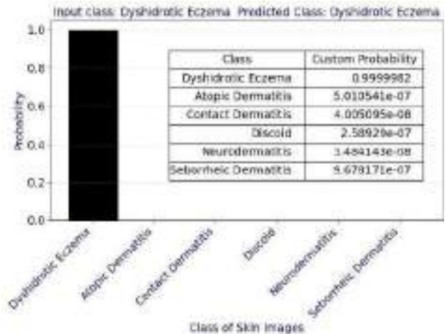
Fig.8(e).ProbabilitiesofClasses
