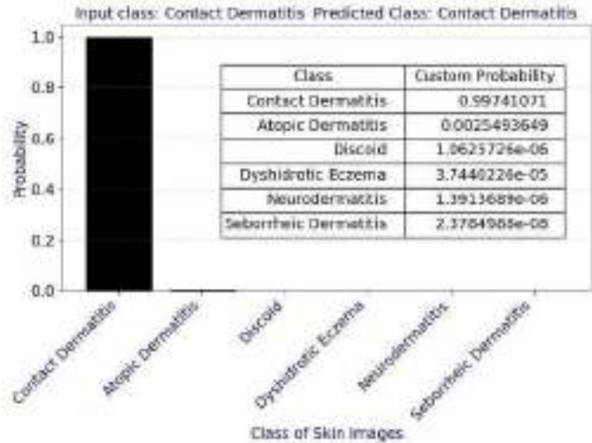
Fig.8(b).ProbabilitiesofClasses
