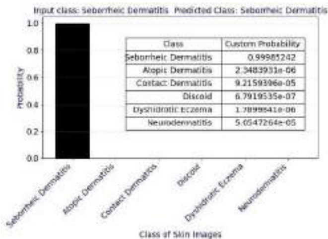
Fig.8(f).ProbabilitiesofClasses
