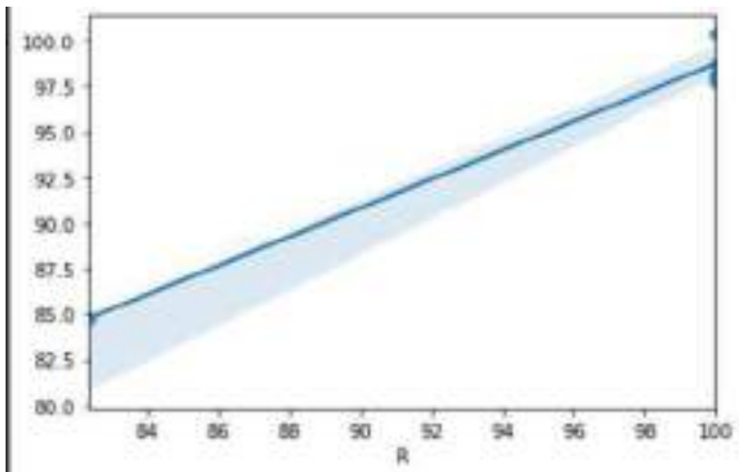
Figure 4. Prediction Plot.
