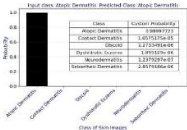
Fig.8(a).ProbabilitiesofClasses
