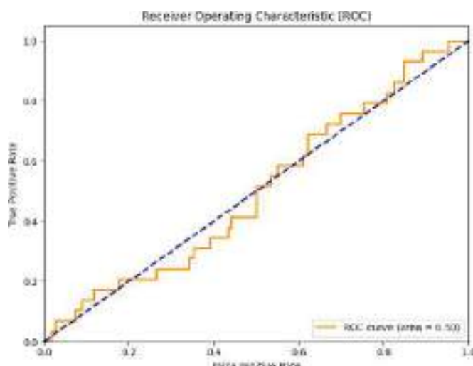
Fig.6.ROCcurve
