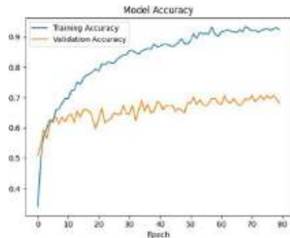
Fig.4. DenseNet-121-Accuracy Plot
