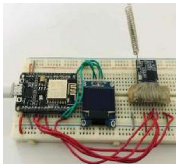
Figure4.1: Hardware Implementation
