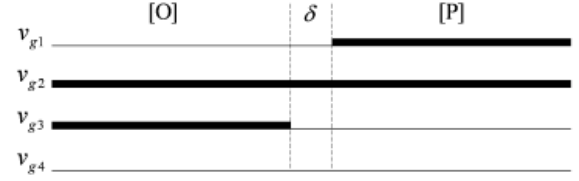
Fig.2.2.a Gate Signals
