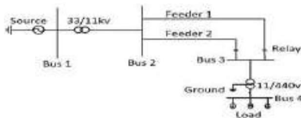
Fig.2 parallel feeder
