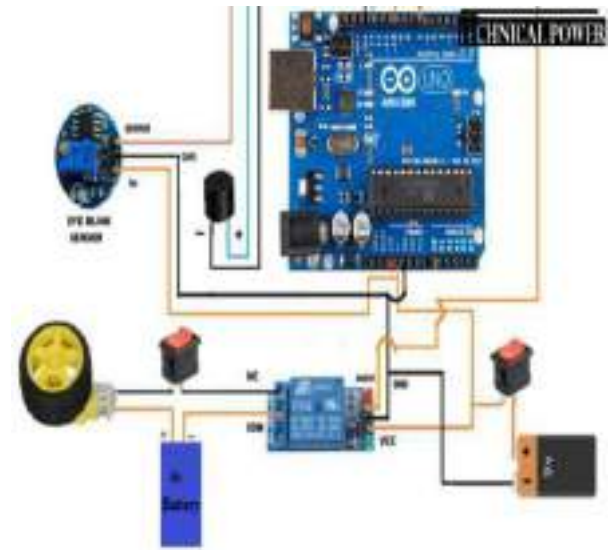
Fig 1. Circuit Diagram
