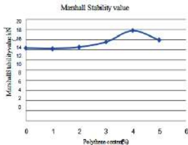
Figure 3: Marshall Stability Value
