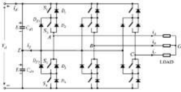
Fig2.1 Three Level NPC Inverter
