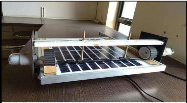
Fig. 4.1 Model of Solar Panel Cleaning System
