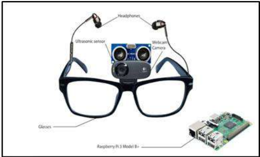
Figure 4. Working Mechanism
