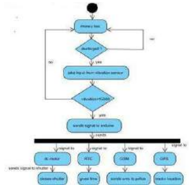
Figure 2: Workflow of the system using Activity diagram
