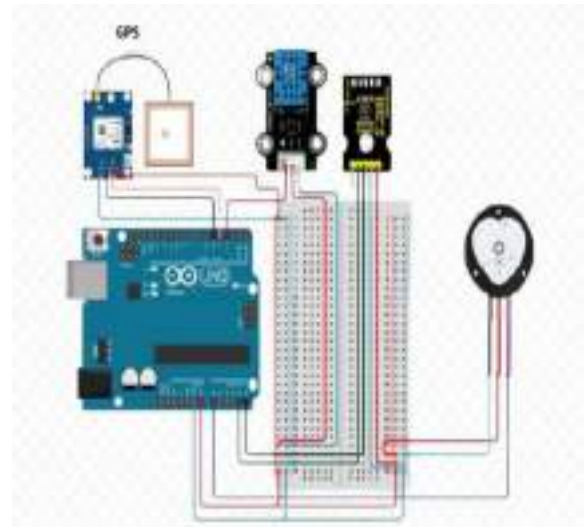
Figure2: Transmitter Side
