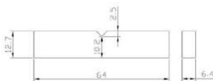
Fig.12: ASTM D 695 standard impact specimen
