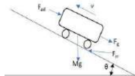
Figure 1. Vehicle dynamics
